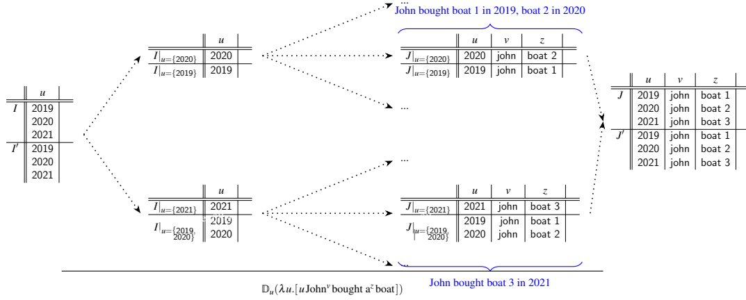
Figure 4: Pair-based distributivity
